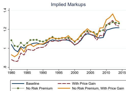
Figure A.5: Implied Markups.
