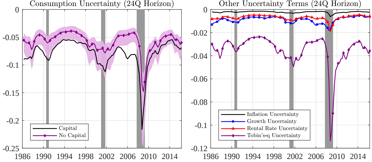
Figure 9: Filtered decomposition of the effects on current consumption. The shaded regions denote NBER recessions. The vertical axis is the contribution to the percentage point deviation of detrended consumption from its steady state.
