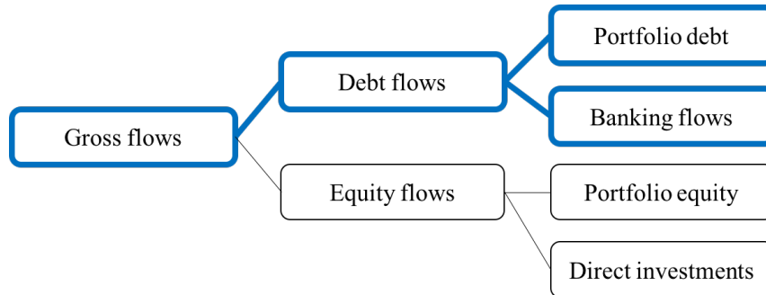
Figure 3: Decomposition of gross flows
