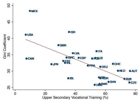
Figure 18: Gini coefficient
