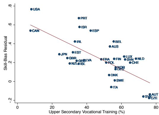
Figure 16: Skill-Bias
