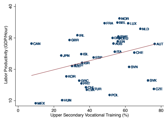
Figure 19: Labor Productivity
