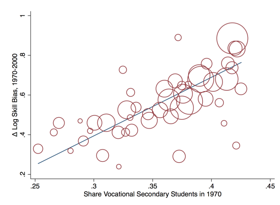
Figure 14: \Delta Skill-Bias
