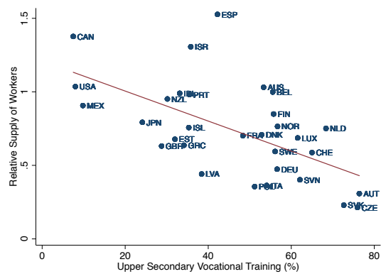
Figure 17: Relative Supply
