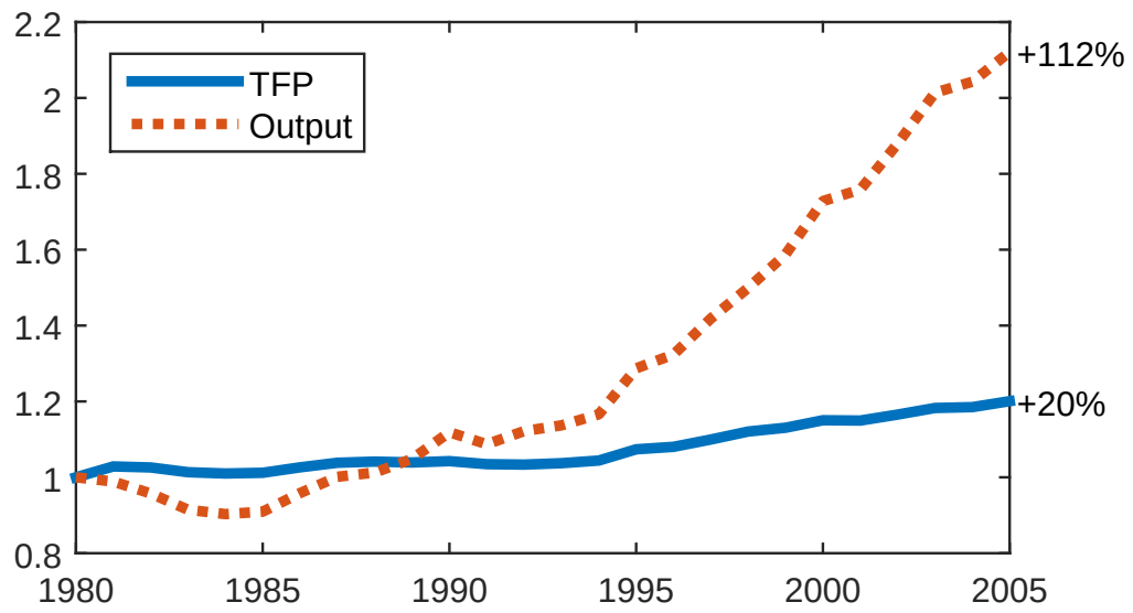
Figure 7. Inferred TFP values
