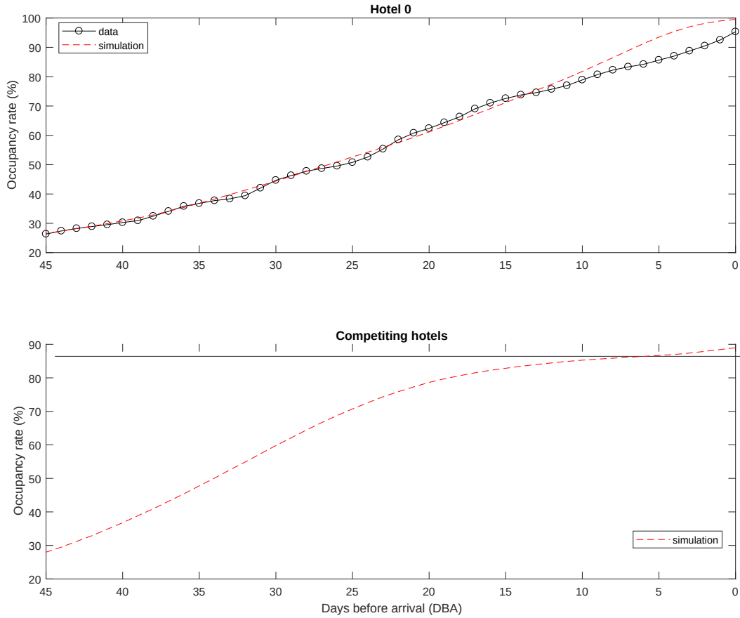
Figure 16: Occupancy trajectory for sample 31, busiest weekend
