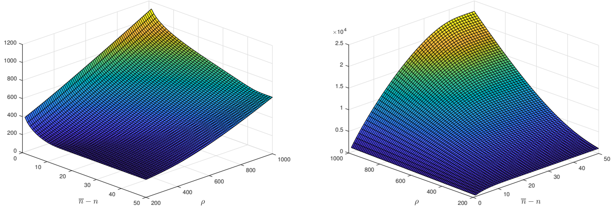
Figure 12: Example of optimal pricing rule p_0^*(n, \rho, \bar{p}) and V_0^f(n, \rho)
