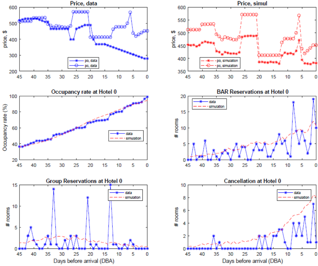
Figure 14: Simulated versus actual outcomes, day 41 of sample20
