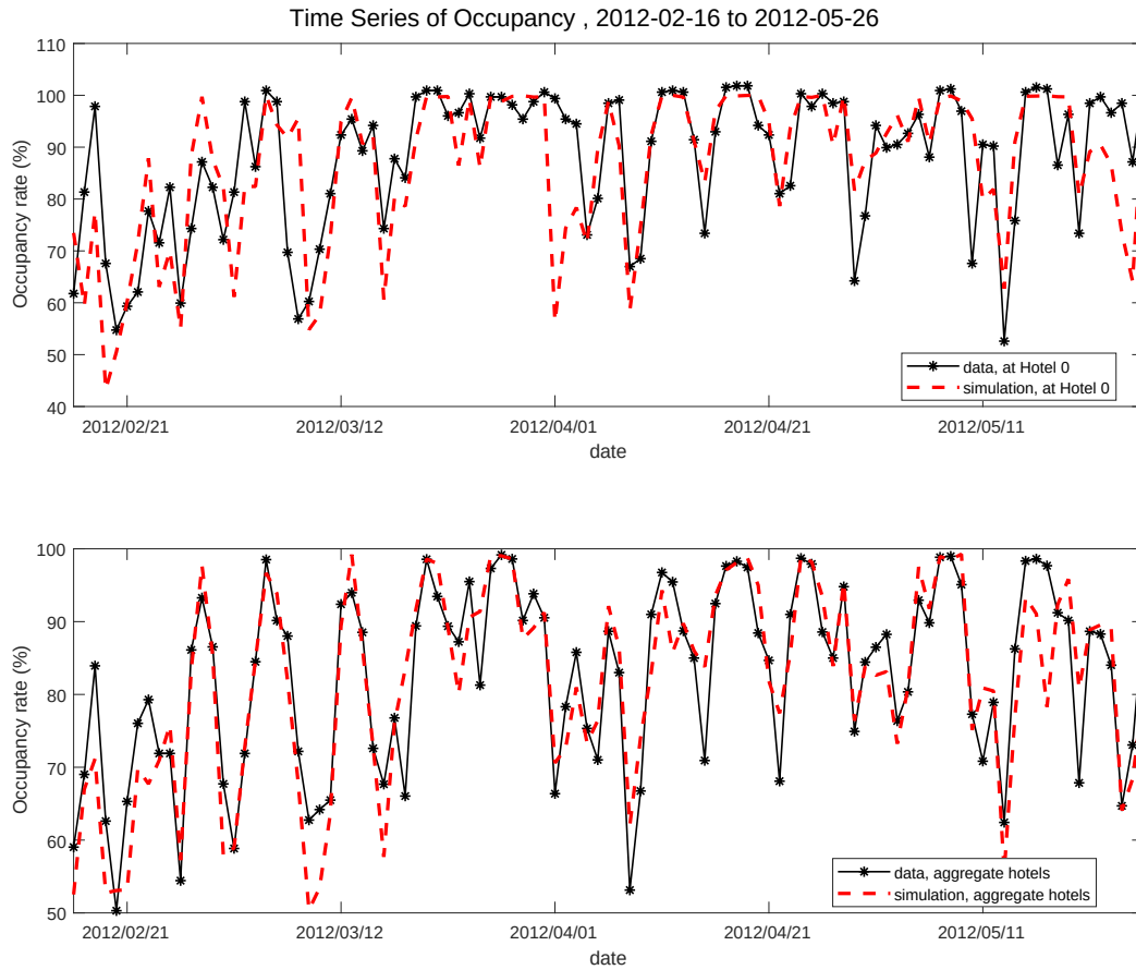
Figure 18: Time Series of Occupancy
