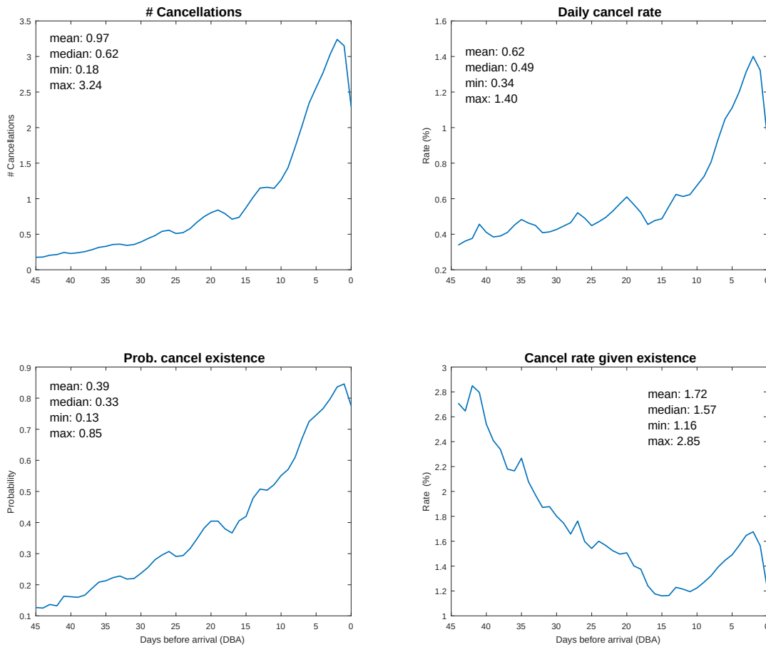
Figure 9: Cancellation dynamics
