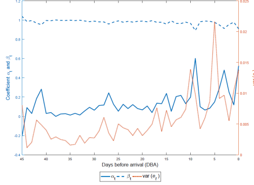
Figure 10: Estimated competitor BAR transition parameters
