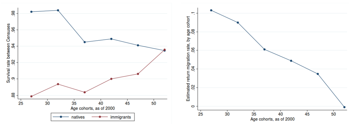
Figure 9: Return migration
