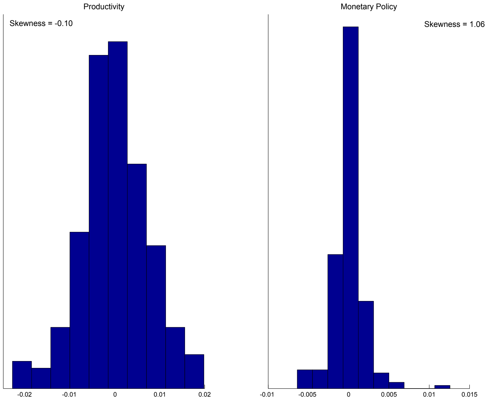
Figure 2: Histogram of Residuals Computed from the U.S. Data
