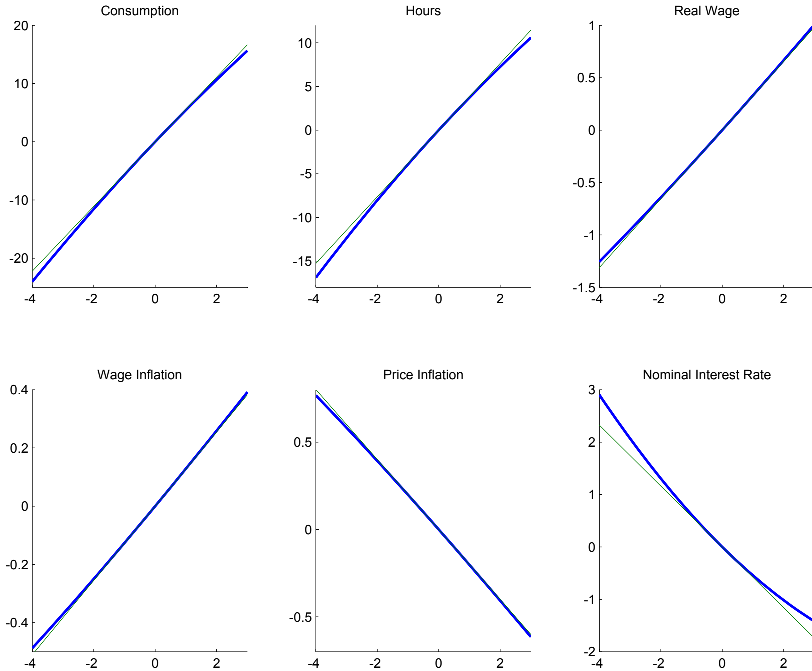
Figure 6: Decision Rules of the Ramsey Planner
