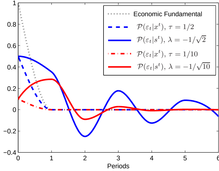
Figure 1: Impulse Responses of x_t and s_t to a one unit change in \varepsilon_t for signal-to-noise ratios of \tau = 1/2 , \lambda = -1/\sqrt{2} (dashed, solid blue) and \tau = 1/10 , \lambda = -1/\sqrt{10} (dashed-dot, solid red). The black dotted line is the innovation itself, \varepsilon_t , normalized to 1.
