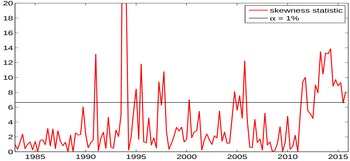
Figure 4: Test for the null that the distribution of the individual Blue Chip nowcasts is symmetric.
