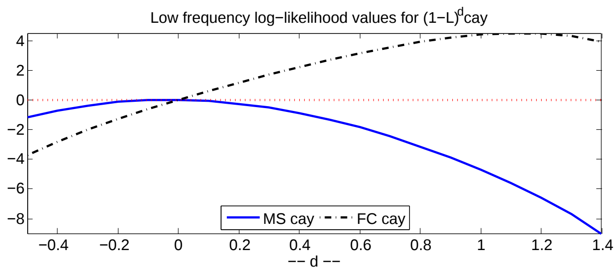
Figure 5: Low frequency log likelihood values for (1 - L)^d cay_t . The sample is quarterly and spans the period 1952:Q1 to 2013:Q3.
