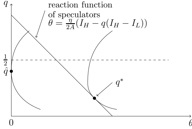
Figure 2: q^* < \hat{q}
