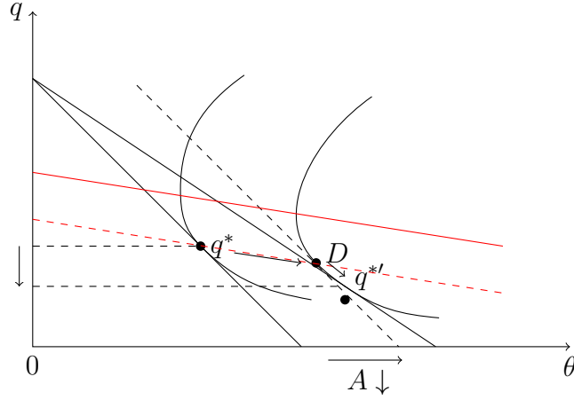
Figure 5: Graphic illustration of Implication 1
