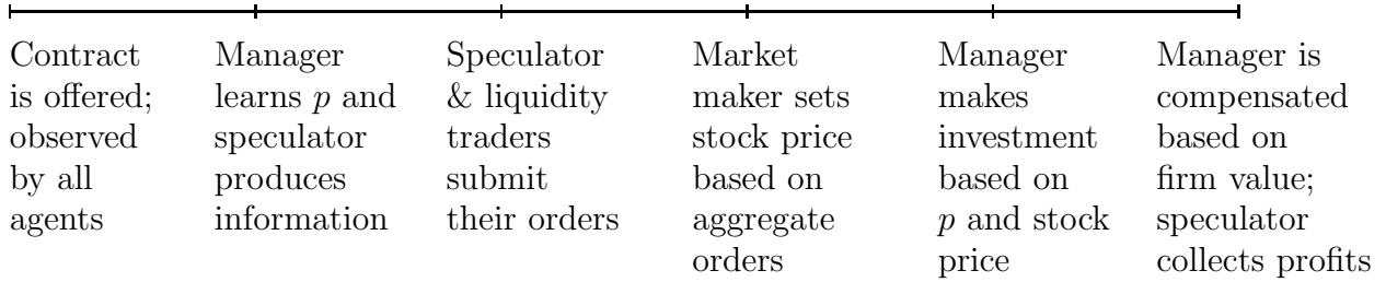
Figure 1: Model Timeline
