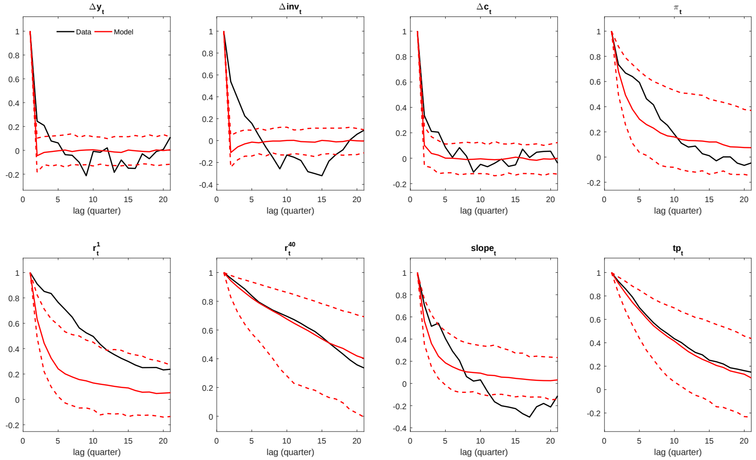
Figure 1: Autocorrelation Functions
