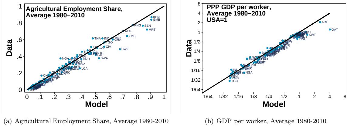
Figure 9: Simulations and data for cross-section of the average for 1980-2010. Line depicts 45 degrees.
