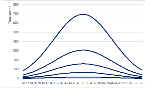
Figure 3: Inheritance Profiles
