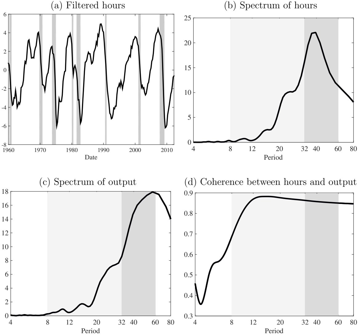
Figure 5: Data, spectral density and coherence
