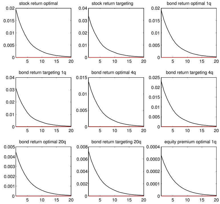
Figure 3: Deviations from steady state after a 1% dividend shock for the stock return under optimal policy, stock return under 2% inflation targeting, 1-quarter bond return under optimal policy, 1-quarter bond return under 2% inflation targeting, 4-quarter bond return under optimal policy, 4-quarter bond return under 2% inflation targeting, 20-quarter bond return under optimal policy, 20-quarter bond return under 2% inflation targeting and equity premium over the 1-quarter bond under optimal policy (Section 5).
