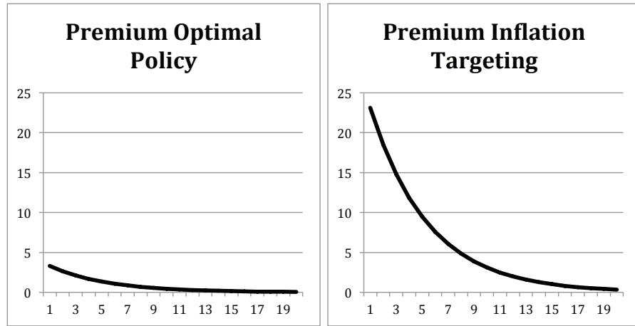
Figure 5: Deviations from steady state after a 1% dividend shock for the equity premium over the 1-quarter bond produced under 2% inflation targeting compared to the optimal policy, in basis points (Section 5).
