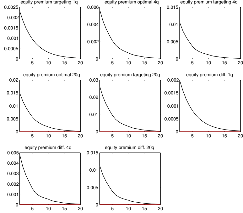
Figure 4: Deviations from steady state after a 1% dividend shock for equity premium over the 1-quarter bond return under 2% inflation targeting, equity premium over the 4-quarter bond return under optimal policy, equity premium over the 4-quarter bond return under 2% inflation targeting, equity premium over the 20-quarter bond return under optimal policy, equity premium over the 20-quarter bond return under 2% inflation targeting, difference in equity premium over the 1-quarter bond produced under 2% inflation targeting compared to the optimal policy, difference in equity premium over the 4-quarter bond produced under 2% inflation targeting compared to the optimal policy and difference in equity premium over the 20-quarter bond produced under 2% inflation targeting compared to the optimal policy (Section 5).
