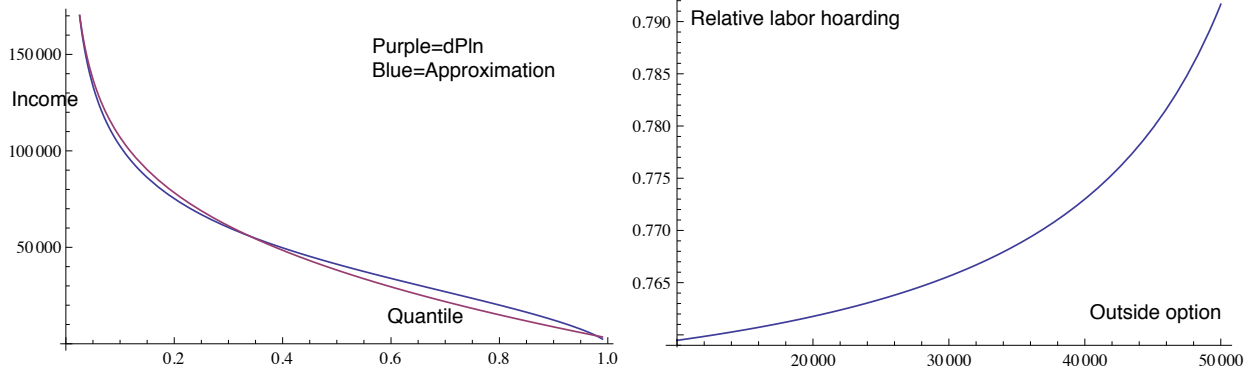
Figure 8: Left: US income distribution approximated by a dPln distribution with parameters (\alpha, \beta, \mu, \sigma) = (3, 1.43, 10.9, .45) (income on the y-axis, quatile on the x-axis) and an approximation to it P(q) = 10^4 \cdot (2.2q^{-.42} + 9.1 - 11q^{.42}) . Right: relative labor hoarding in the SZ model with \lambda = 1 and demand given by the approximation for W_0 \in 10^4 \cdot [1, 5]
