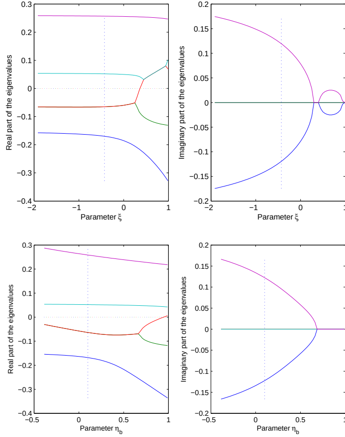
Figure 6: “Node–focus” Bifurcations
