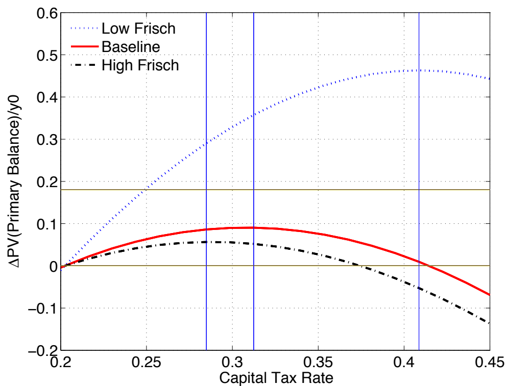
Figure 7: Capital Tax Dynamic Laffer Curves: Different Frisch Elasticities
