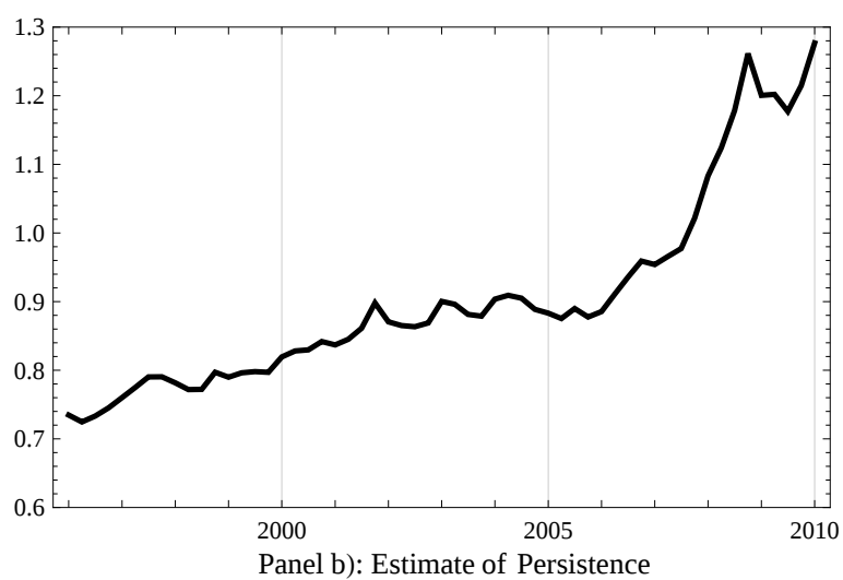
Figure 1: in Panel a) US Household Leverage Ratio 1996Q1-2010Q1 (Source: Boz and Mendoza [5]); in Panel b) Model Estimate of Leverage Autocorrelation 1996Q1-2010Q1; Panel a): Leverage Data
