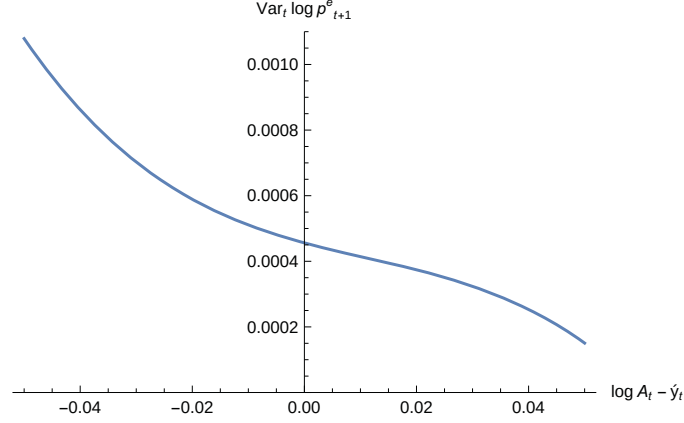
Figure 7. One-step-ahead variance of the log equity price p_t^e in the baseline model computed to fifth order. Low values of A_t relative to \bar{y}_t correspond to a weaker economy, and to a more volatile equity price. See text for details.
