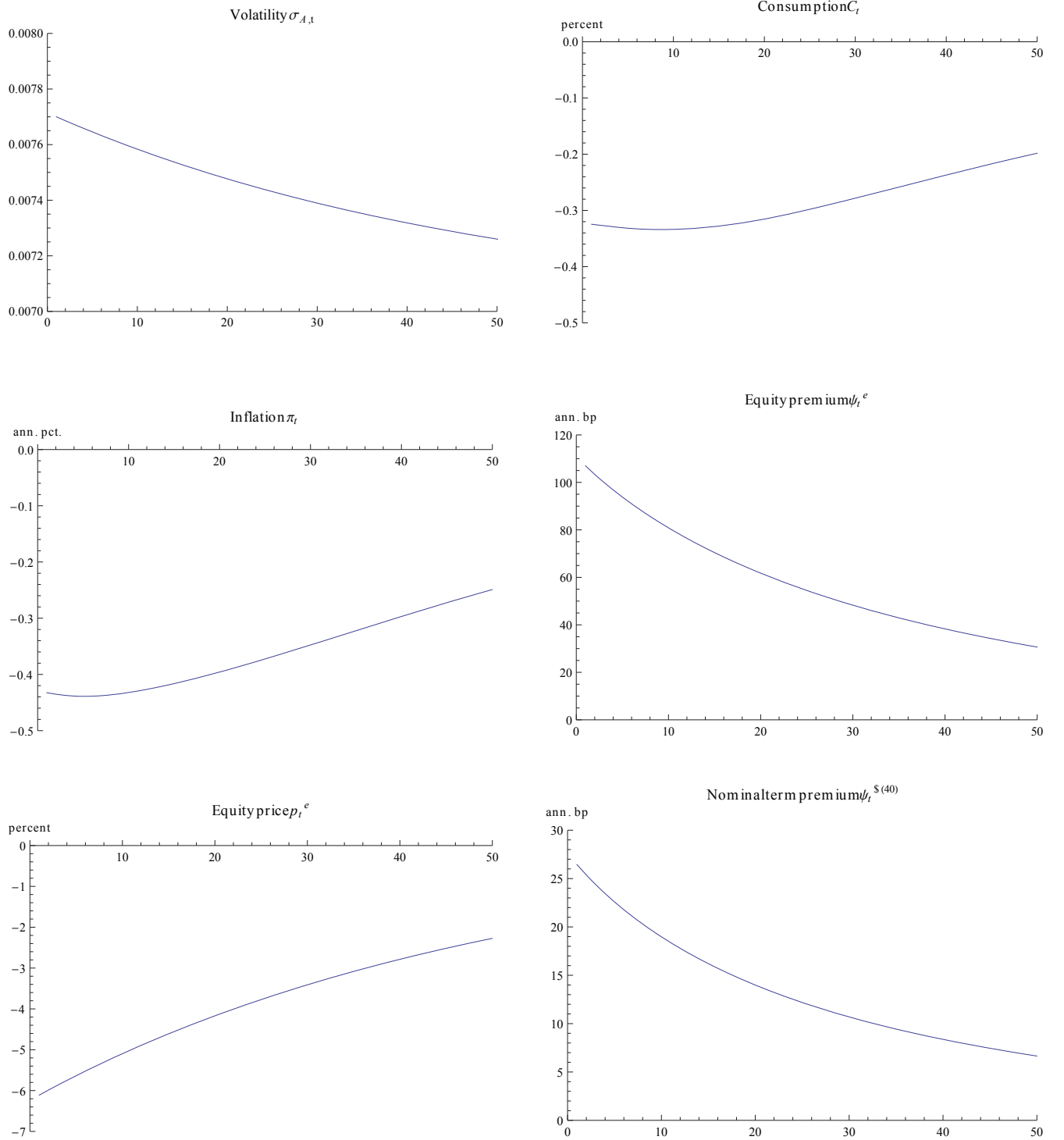
Figure 6. Nonlinear impulse response functions for volatility \sigma_t^A , consumption C_t , inflation \pi_t , the equity premium \psi_t^e , equity price p_t^e , and nominal term premium \psi_t^{S(40)} to a one-standard-deviation (0.1 percent, or .0007) volatility shock in the extended model. See text for details.
