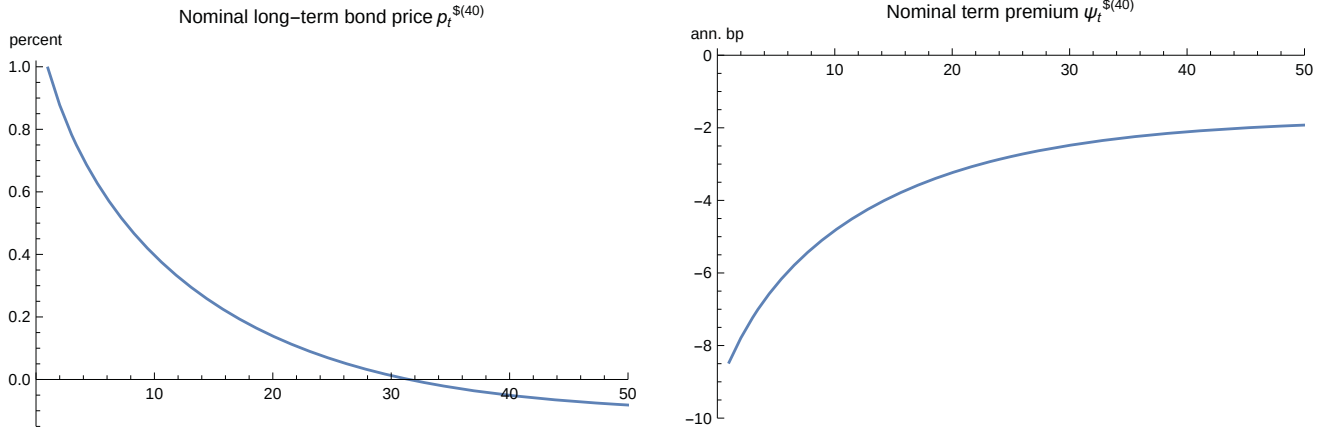
Figure 4. Nonlinear impulse response functions for nominal long-term bond price p_t^{$(40)} and term premium \psi_t^{$(40)} to a one-standard-deviation (0.7 percent) technology shock in the model, with state variables initialized to their nonstochastic steady state values. See text for details.
