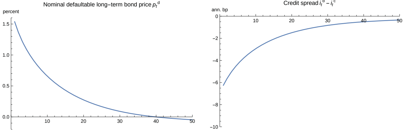
Figure 5. Nonlinear impulse response functions for defaultable long-term bond price p_t^d and credit spread i_t^d - i_t^c to a one-standard-deviation (0.7 percent) technology shock in the model, with state variables initialized to their nonstochastic steady state values. See text for details.
