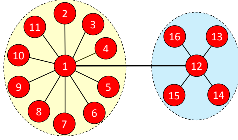
FIGURE 2. Center-connected local stars, in a context with two groups.
