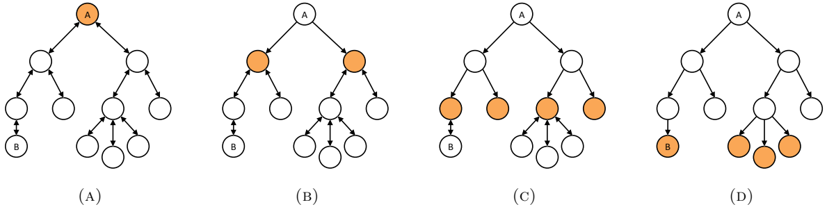
FIGURE 4. As the algorithm progresses, directed links into nodes that are reached are deleted. This ensures that only minimal paths are included. In this case, as in all tree networks, there is a unique minimal path from A to B.
