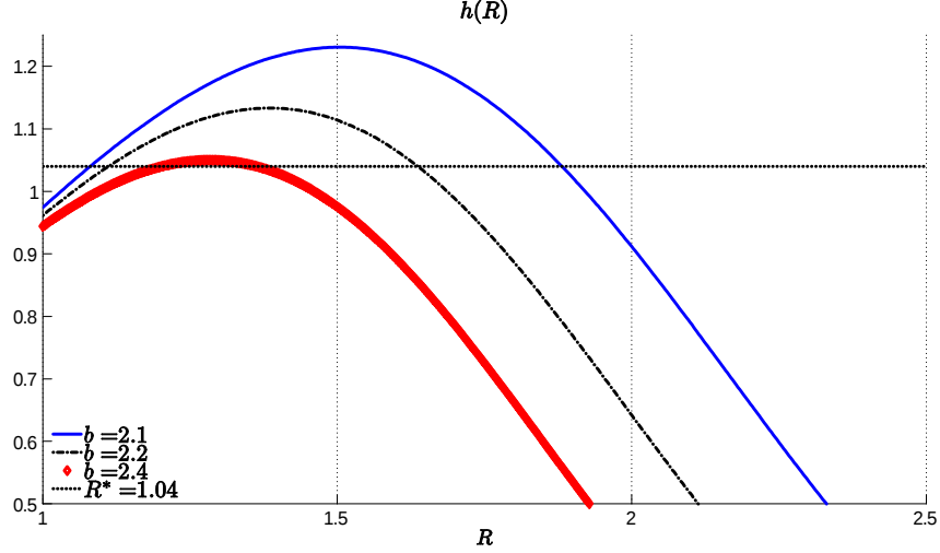
Figure 1: Expected return h(R; b)
