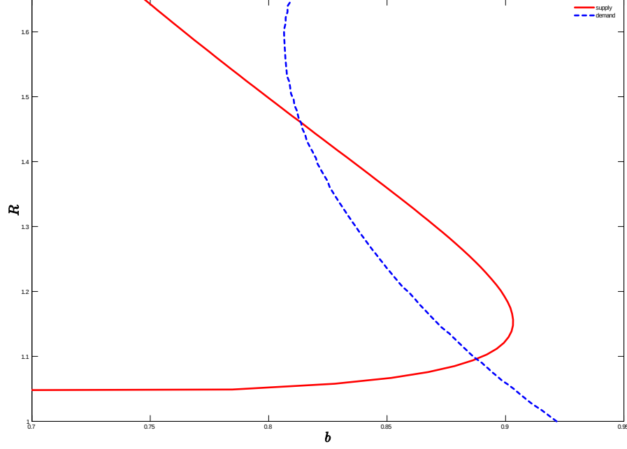
Figure 3: Supply and demand curves
