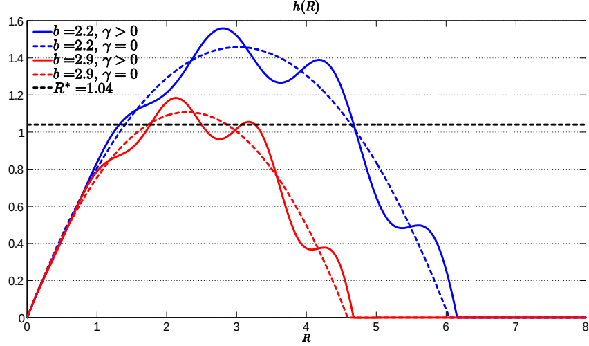
Figure 7: Perturbing the uniform distribution
