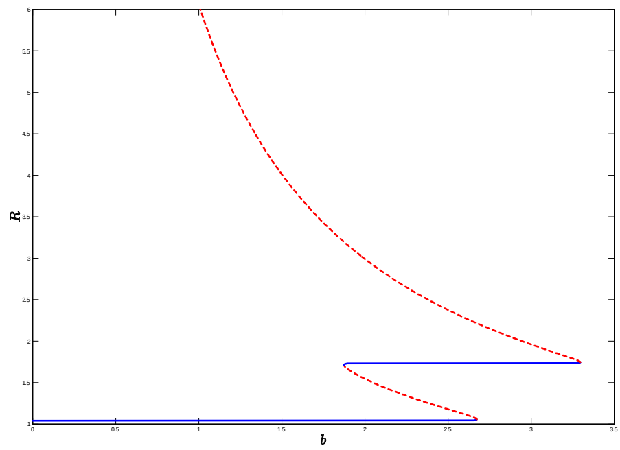
Figure 5: Interest rate schedules for the bimodal distribution
