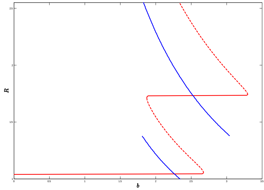
Figure 6: Supply and demand for the bimodal distribution
