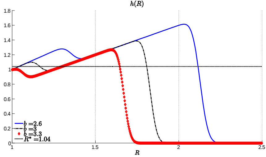
Figure 4: Expected return for the bimodal distribution
