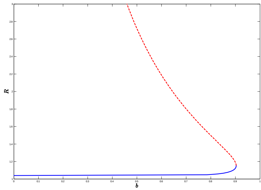
Figure 2: Interest rate schedules
