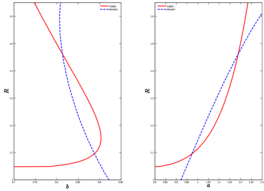
Figure 8: b and a schedules
