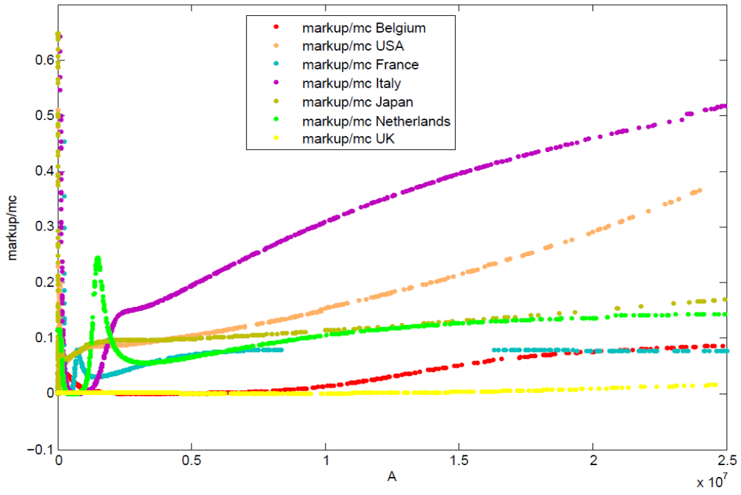
FIGURE 9: Markup to Base Marginal Cost Ratio for All Countries
