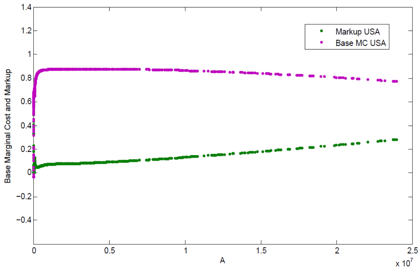
FIGURE 8: Estimates of \hat{c}_{ni}^{\infty,A}(\cdot) and Markup for US
