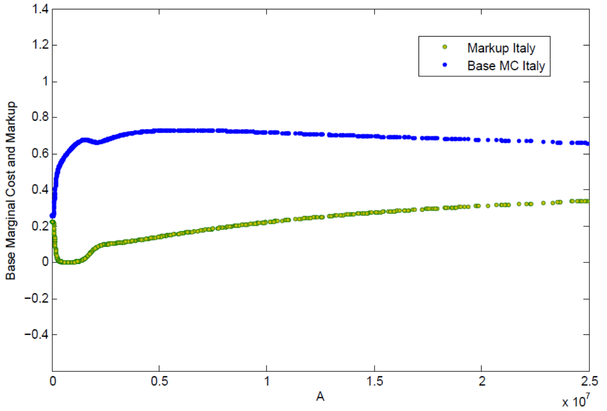
FIGURE 4: Estimates of \hat{c}_{ni}^{\circ,A}(\cdot) and Markup for Italy
