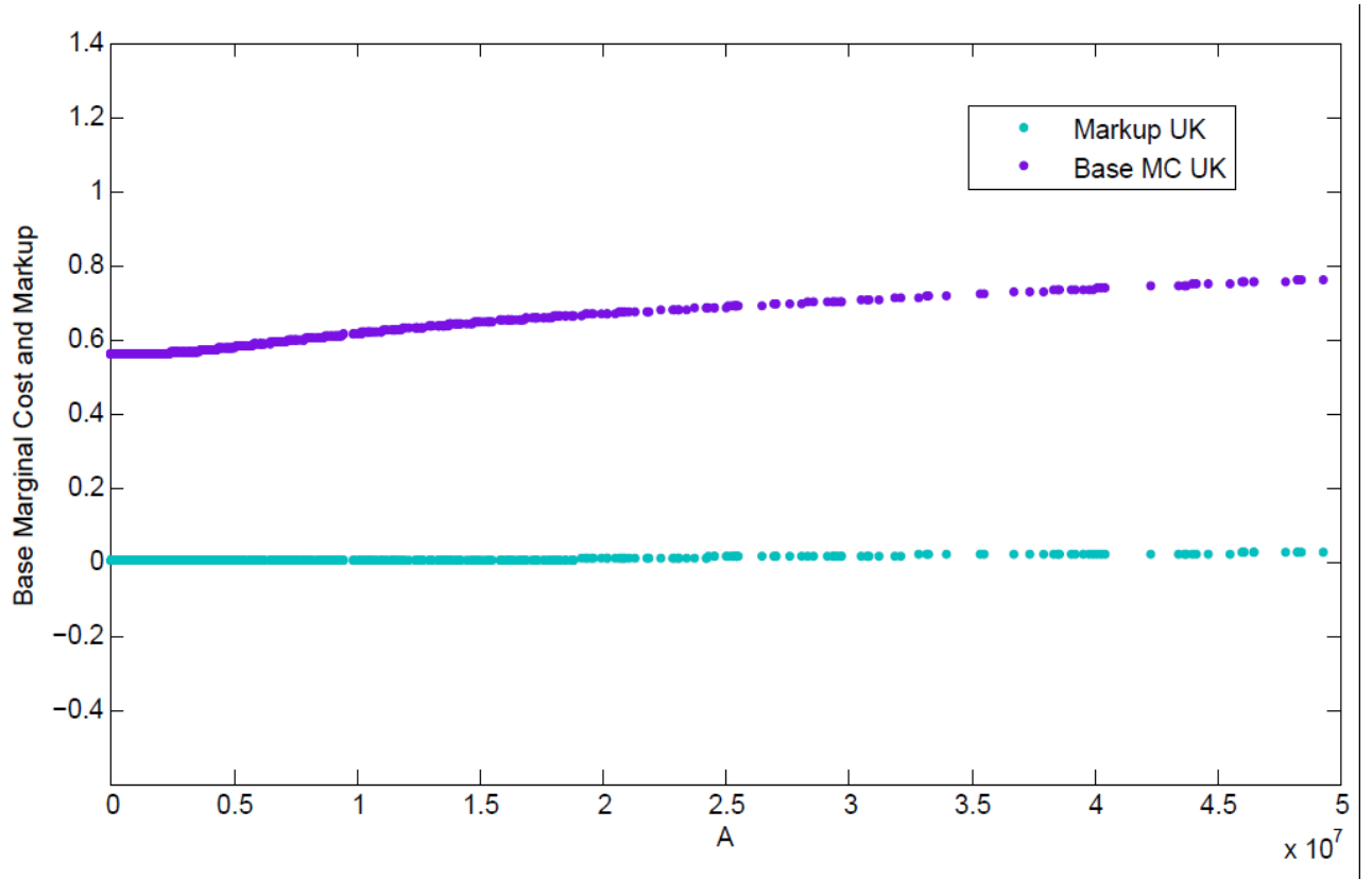
FIGURE 7: Estimates of \hat{c}_{ni}^{\infty,A}(\cdot) and Markup for UK
