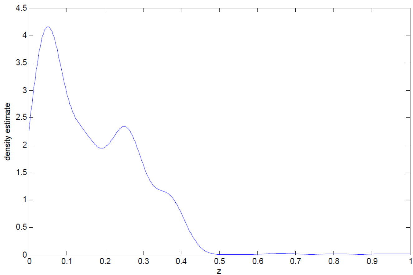
FIGURE 12: Estimated density \hat{f}_{ni}(\cdot) for Italy
