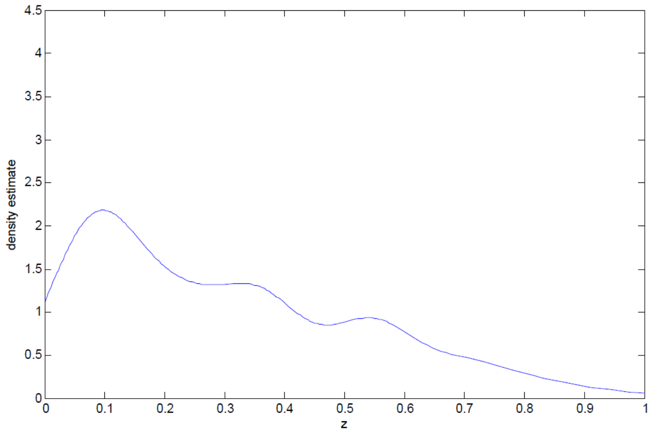
FIGURE 11: Estimated density \hat{f}_{ni}(\cdot) for France
