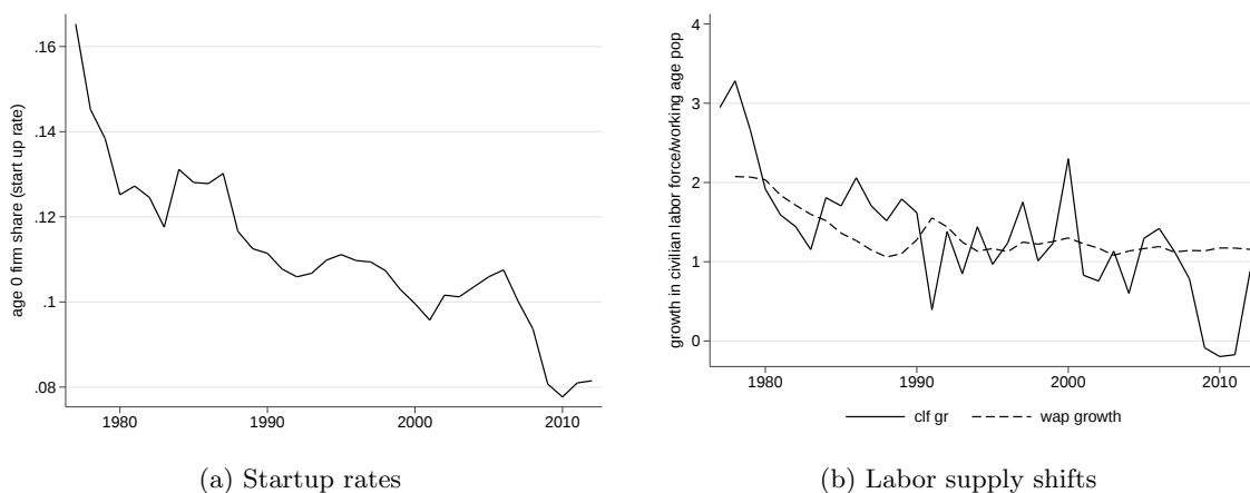
Figure 1: Declines of startup rate and labor supply growth rate from 1977 to 2012
