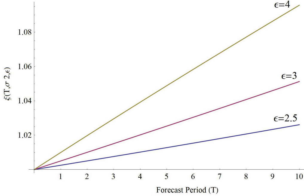
Figure 1 Behavior of Amplifying Curvature Term: \xi(T, \sigma, \epsilon)
