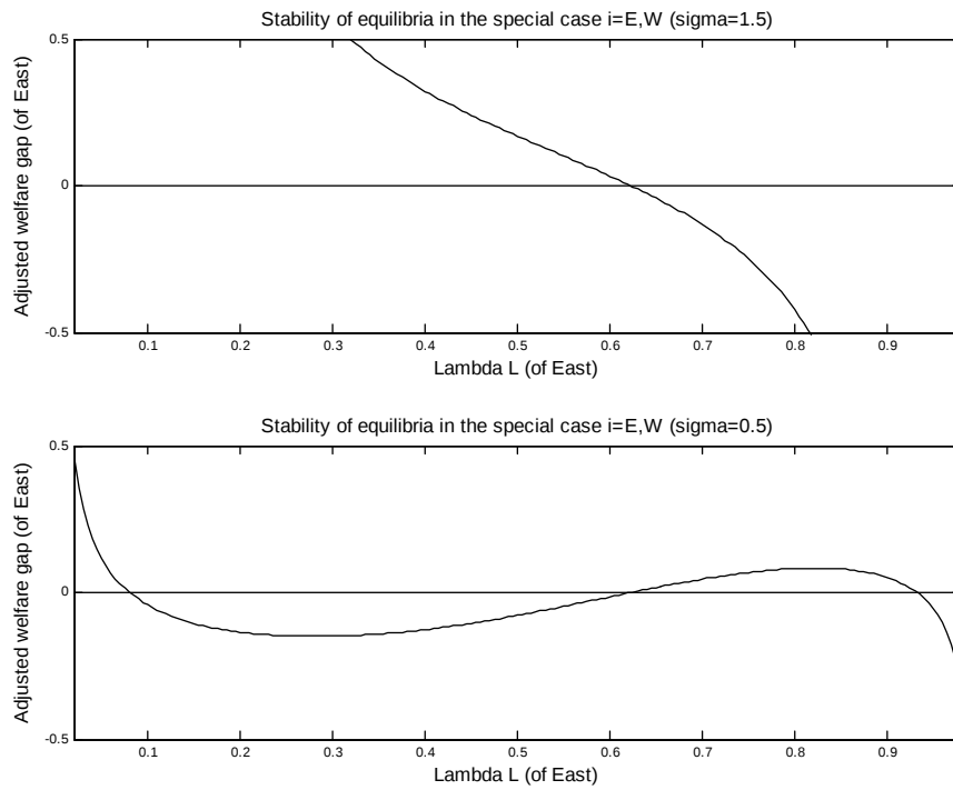
Figure 10: Stability of equilibria in the two-region case
