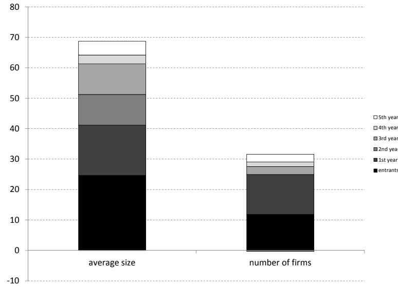
Figure 3: Variance decomposition
