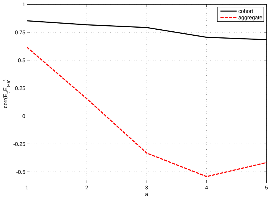
Figure 2: Autocorrelations
