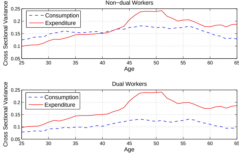
Figure 4: Household Composition: Data
