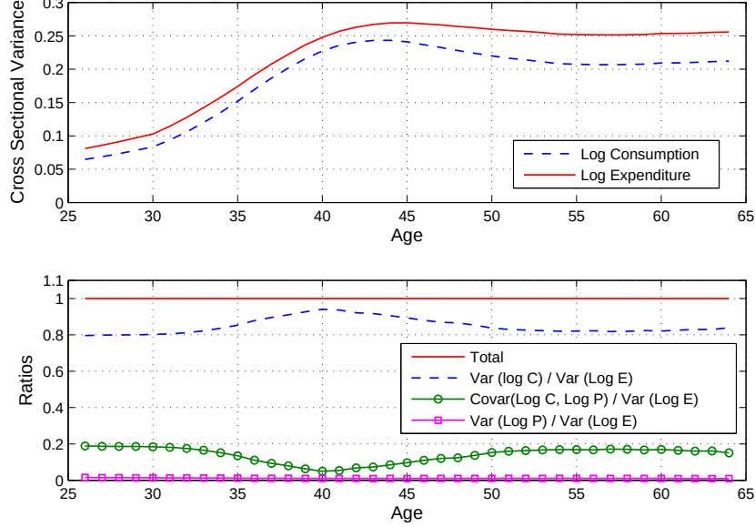
Figure 2: Cross Sectional Variance: Consumption vs Expenditure
