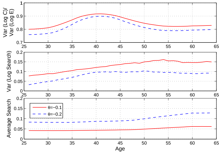
Figure 7: Effect of Price Search Technology
