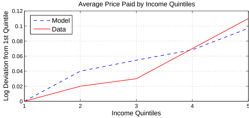
Figure 3: Labor Income and Prices: Model vs Data
