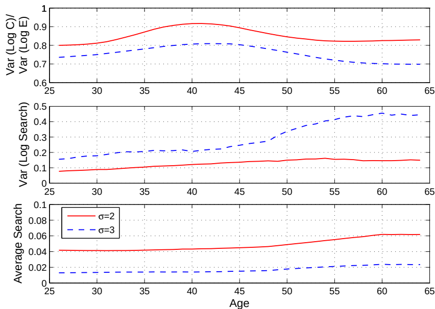
Figure 6: Effect of Risk Aversion
