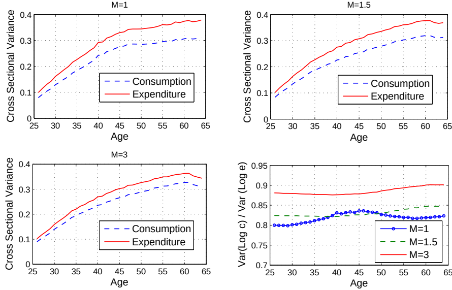
Figure 5: Household Composition: Model
