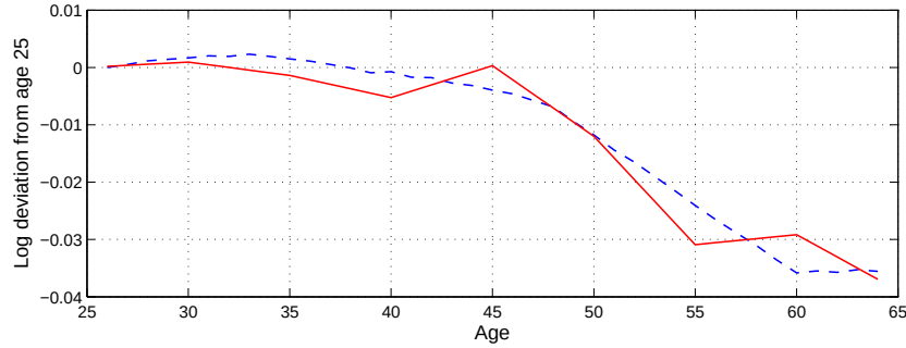
Figure 1: Life-cycle profile of Prices: Model vs Data
