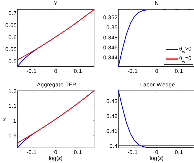
Figure 4: Effect of aggregate TFP z on output Y , employment N , measured TFP Y/N^\alpha , and the measured labor wedge.
