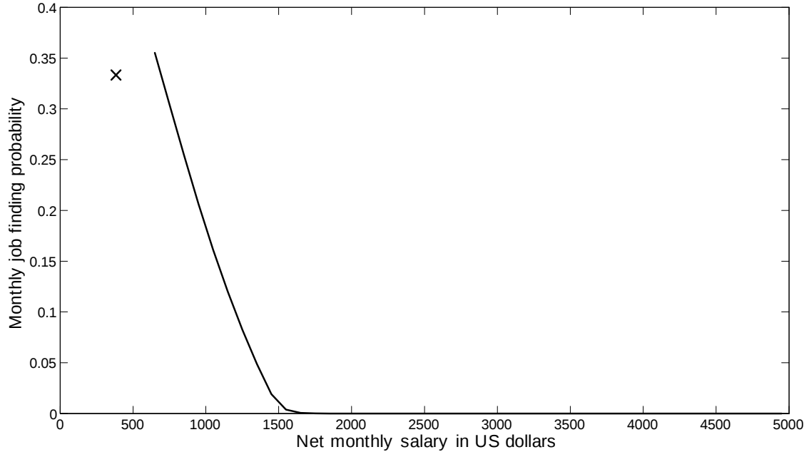
Figure 3: Search intensity
