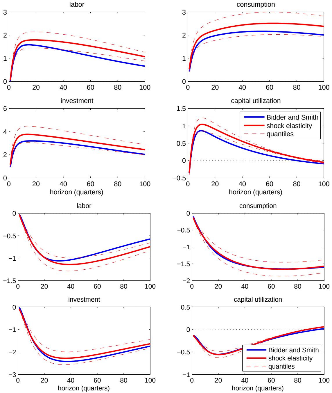
Figure 2: A comparison of shock elasticities computed using the second-order robust preference expansion method from this paper with the results from Bidder and Smith (2012) . Top four graphs present responses to the technology shock, bottom four graphs responses to the volatility shock. Shock elasticities computed under the worst-case model, and the mean and quantiles of the responses are conditioned on the stationary distribution under the worst-case model.
