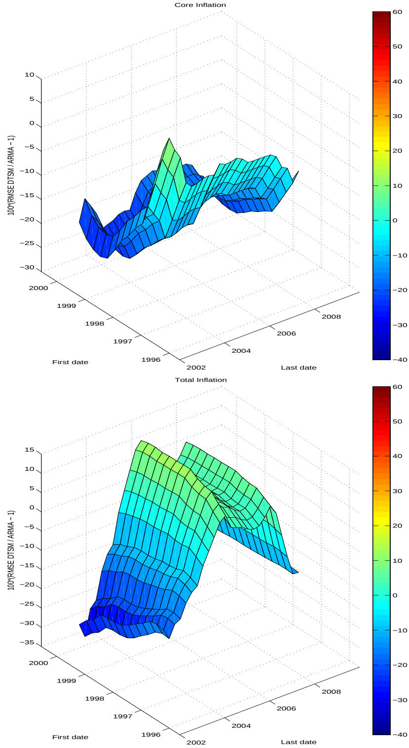
Figure 2: RMSE Percentage Ratios: DTSM 3,3 . For the DTSM 3,3 and ARMA models, we compute RMSEs over a grid of out-of-sample windows with start date ranging from 1996Q4 to 1999Q4 and end date from 2002Q4 to 2008Q4. The figure displays their percentage ratio, 100 \times (\text{RMSE DTSM}_{3,3} / \text{RMSE ARMA} - 1) . Negative numbers in the plot signal that the DTSM outperforms the ARMA.
