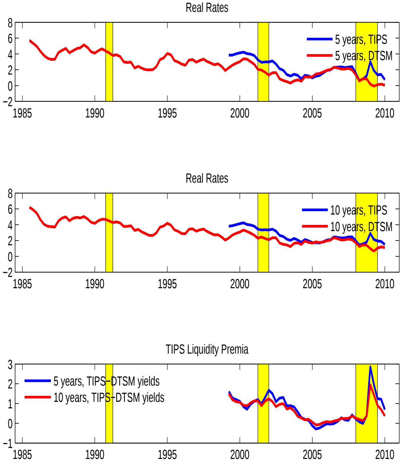
Figure 7: Real Rates: TIPS vs. DTSM. The plots contrast model-implied and TIPS real rates with five and ten years maturity. We compute real rates using a DTSM_{3,3}^* in which level is the only priced risk factor. We estimate the model on the first four principal components of CMT yields with maturities up to ten years and CPI inflation data. The sample period is 1985Q1-2009Q4. The shading corresponds to NBER recessions.
