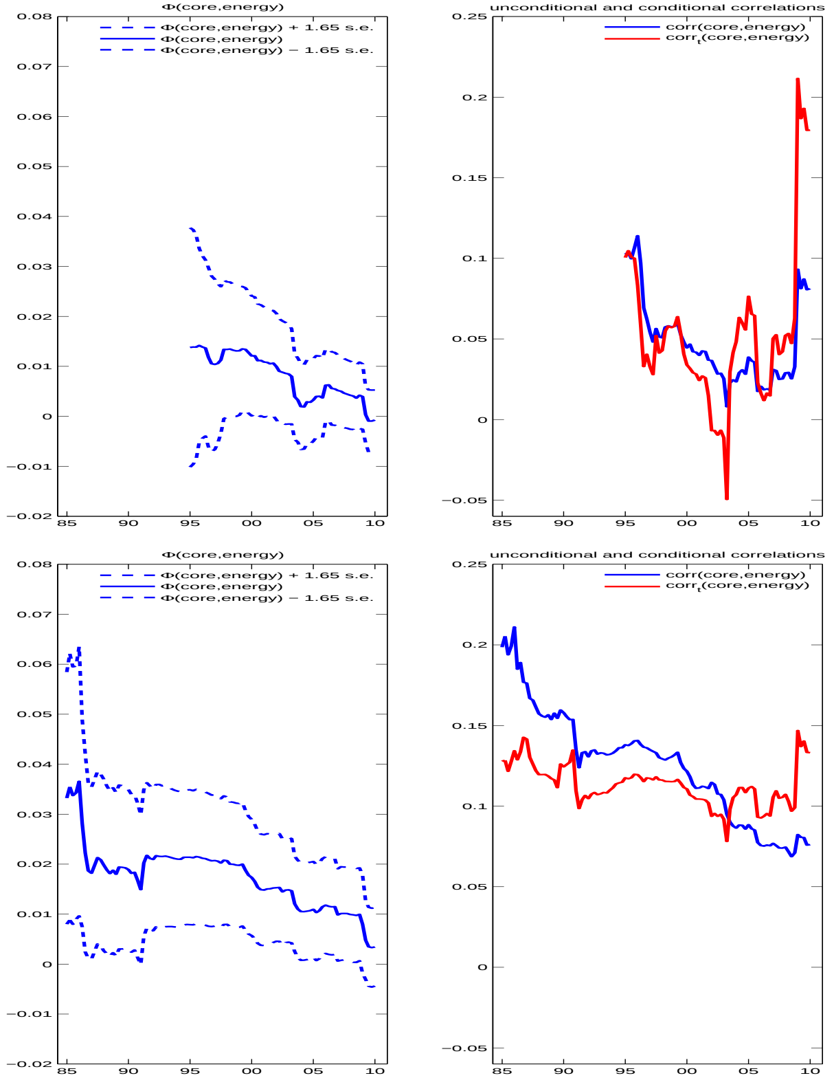
Figure 9: Energy Pass Through. The plots depict measures of correlation between energy and core inflation for a \text{DTSM}_{3,3} . We estimate the model on the first four principal components of CMT yields with maturities up to ten years and CPI inflation data. In the top panels, the sample period starts in 1985Q1 and the end date ranges from 1995Q1 to 2009Q4. In the bottom panels, the sample period starts in 1962Q1 and the end date ranges from 1985Q1 to 2009Q4. The left panels show the estimate for the \phi_1^{\pi^c, \pi^e} coefficient and its 90% confidence bands. The right panels depict conditional and unconditional correlations between core and energy inflation.
