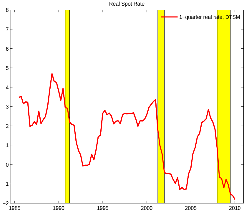
Figure 6: Real Spot Rate. The plot shows the model-implied real one-quarter rate computed using a DTSM_{3,3}^* in which level is the only priced risk factor. We estimate the model on the first four principal components of CMT yields with maturities up to ten years and CPI inflation data. The sample period is 1985Q1-2009Q4. The shading corresponds to NBER recessions.
