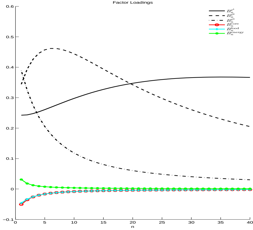
Figure 5: Factor Loadings. The plot depicts the factor loading for nominal yields on the latent factors ( B_n^{\ell^k}, k = 1, \dots, K_1 ) and inflation factors ( B_n^{core} , B_n^{food} , and B_n^{energy} ). We scale the factor loadings to correspond to one standard deviation movement in the factors and we annualize them by multiplying by 400. The sample period is 1985Q4-2009Q4.
