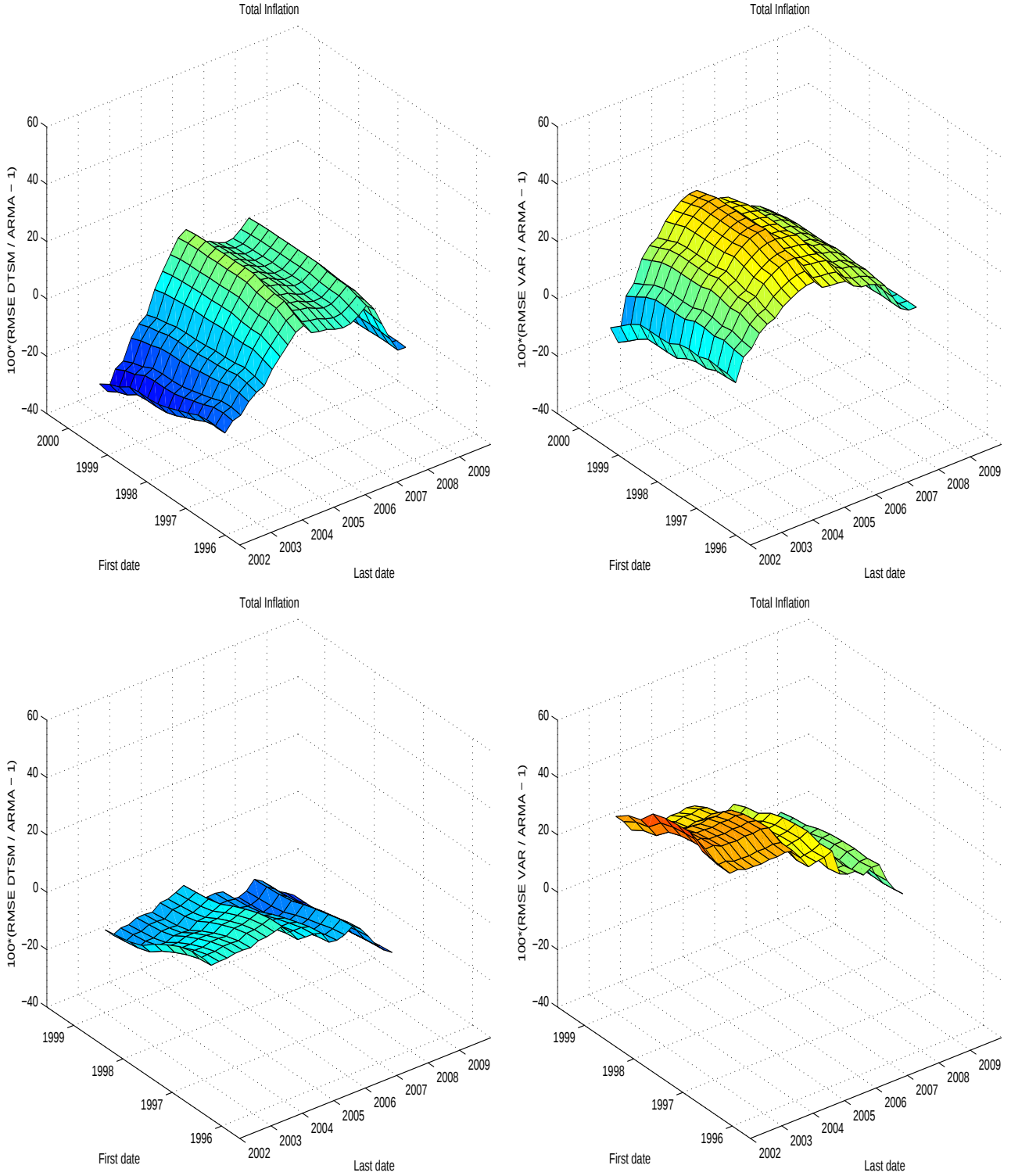
Figure 4: RMSE Percentage Ratios: DTSM 3,3 vs. VAR. We compute RMSEs for the DTSM 3,3 , the unconstrained VAR, and the ARMA(1,1) total inflation forecasts over a grid of out-of-sample windows with start date ranging from 1996Q4 to 1999Q4 and end date from 2002Q4 to 2008Q4. The figure displays the percentage ratios 100 \times (\text{RMSE DTSM}_{3,3} \text{ or VAR} / \text{RMSE ARMA} - 1) . In the left panels, the percentage ratio has the RMSE for DTSM 3,3 in the numerator; in the right panels, it has the RMSE for the VAR. Negative numbers in the plot signal that the DTSM 3,3 / VAR models outperforms the ARMA. In the top panels, the sample period is 1985Q1-2009Q4; in the bottom panels, it is 1962Q1-2009Q4
