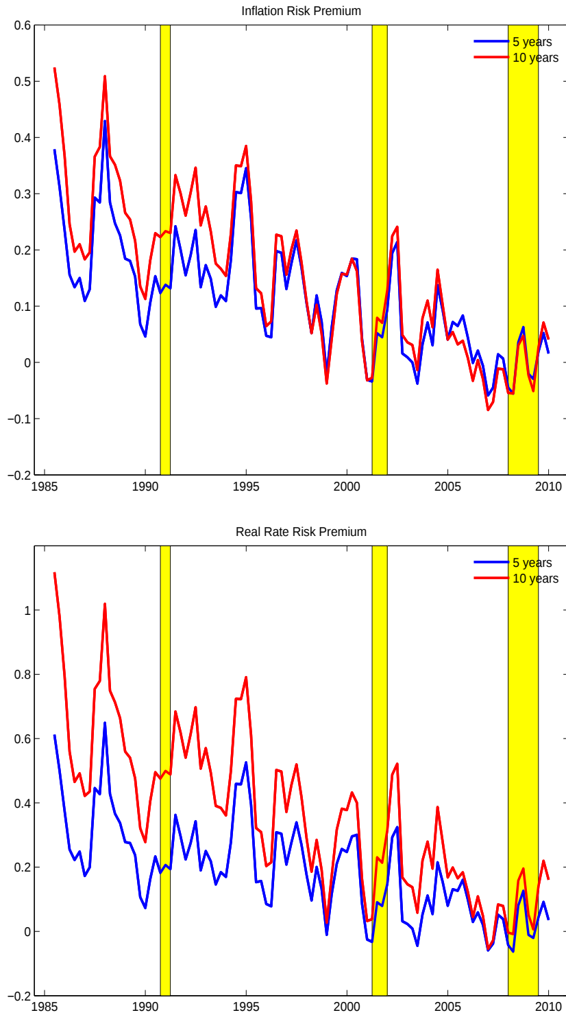
Figure 8: Inflation and Real Rate Risk Premium. The plots depict the five- and ten-year inflation and real rate risk premia implied by a DTSM_{3,3}^* in which level is the only priced risk factor. We estimate the model on the first four principal components of CMT yields with maturities up to ten years and CPI inflation data. The sample period is 1985Q1-2009Q4. The shading corresponds to NBER recessions.
