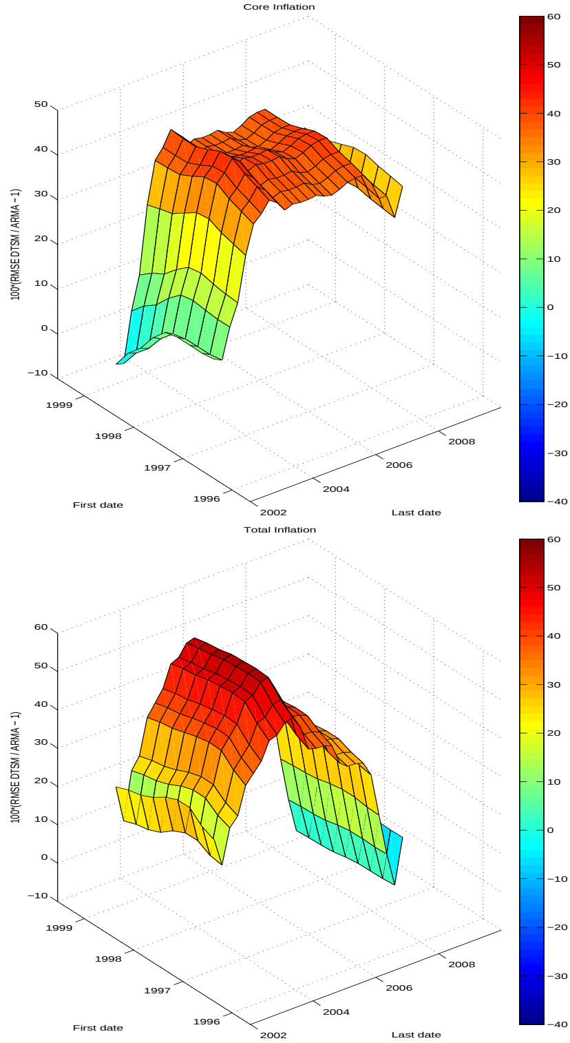
Figure 3: RMSE Percentage Ratios: DTSM 2,1 . For the DTSM 2,1 and ARMA models, we compute RMSEs over a grid of out-of-sample windows with start date ranging from 1996Q4 to 1999Q4 and end date from 2002Q4 to 2008Q4. The figure displays their percentage ratio, 100 \times (\text{RMSE DTSM}_{3,3} / \text{RMSE ARMA} - 1) . Negative numbers in the plot signal that the DTSM outperforms the ARMA.
