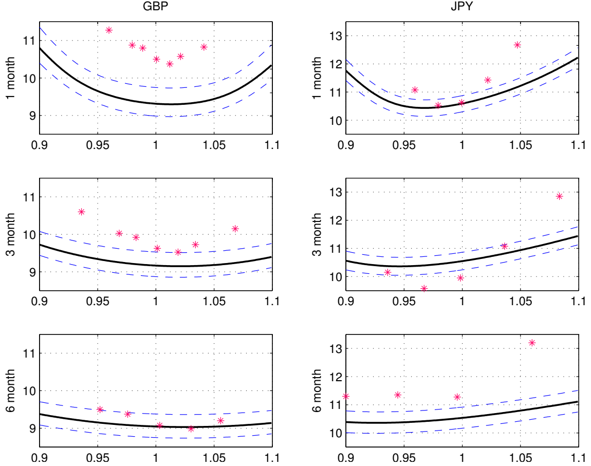
Figure 7: Implied volatility
