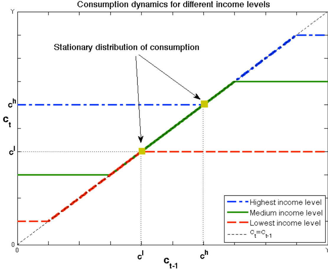
Figure 1: The interval for state s^m overlaps with the the intervals for state s^h and s^l
