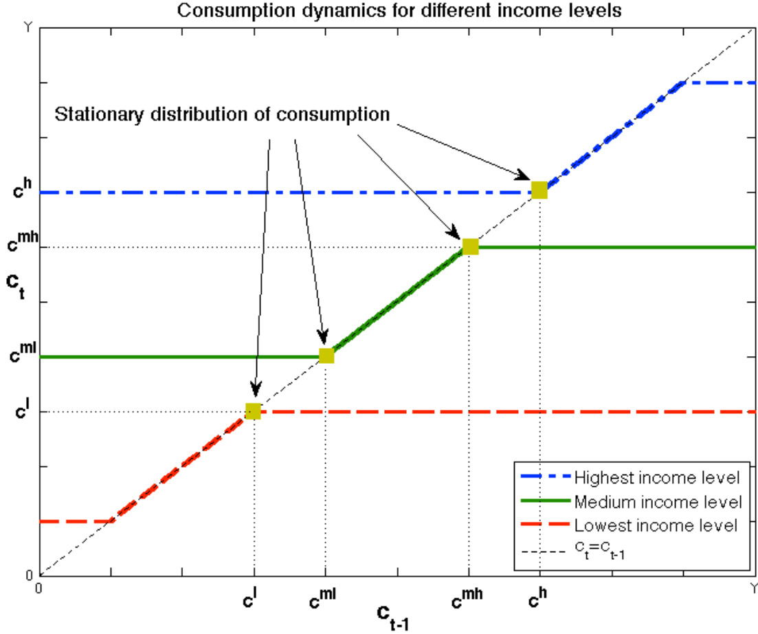
Figure 2: The state-dependent intervals are all disjunct
