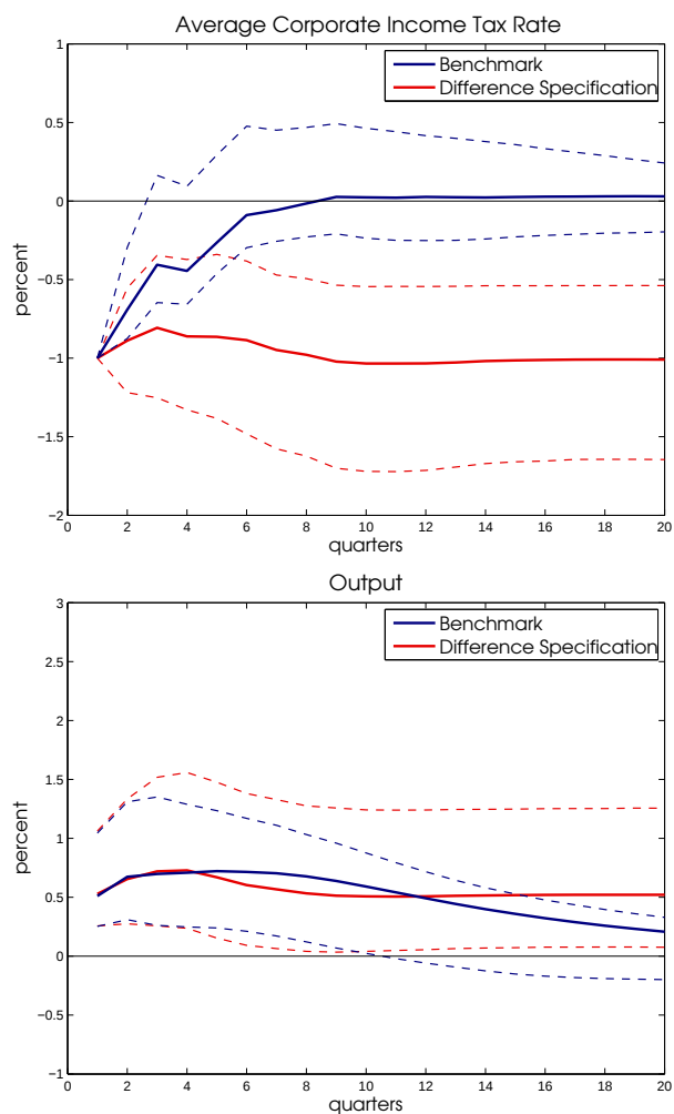
Figure 4 Comparing to a Difference Specification. Broken lines are 95% intervals.
