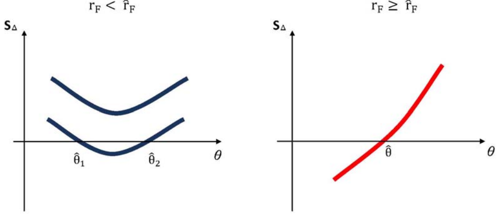
Figure 5: S_\Delta as a function of \theta
