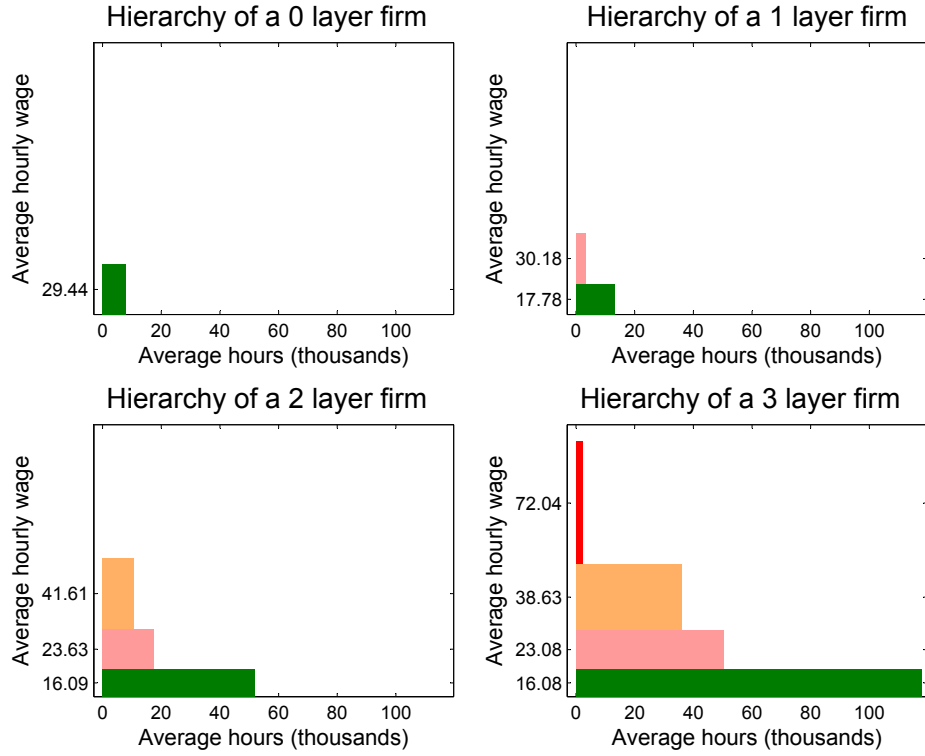
Figure 5: Representative hierarchies
