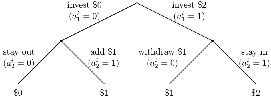
Figure 1: Dynamic investment problem.
