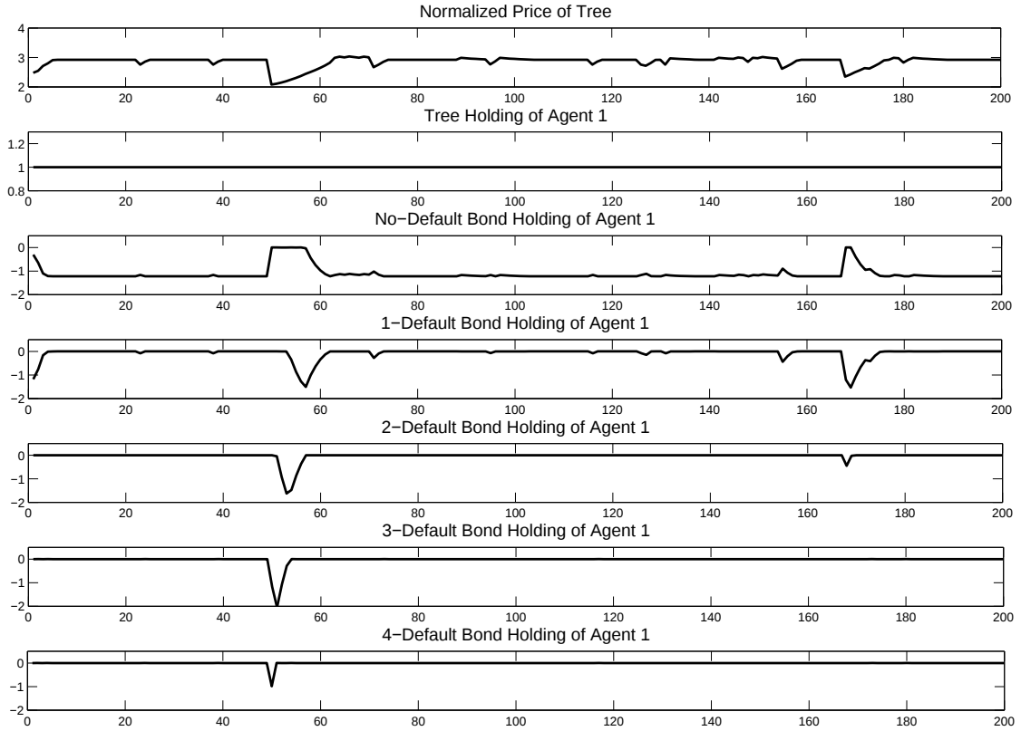
Figure 3: Snapshot from a simulation of the model with 1 tree and 5 bonds
