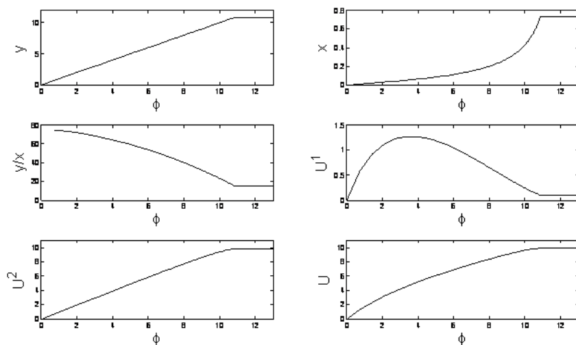
Figure 10: Example 1 continued
