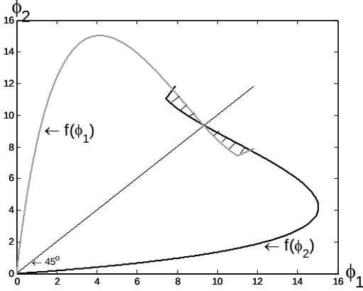
Figure 9-1 Nash sunspot equilibria
