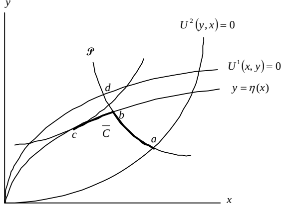
Figure 2-1: Repayment loose
