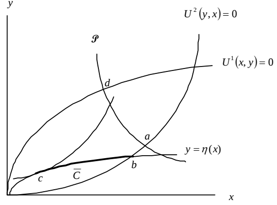
Figure 2-2: Repayment tight
