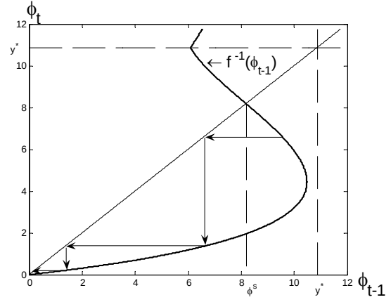
Figure 4-2: Nonstationary equilibria
