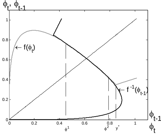
Figure 6-1: Walras cycle, \phi^1, \phi^2 < y^*
