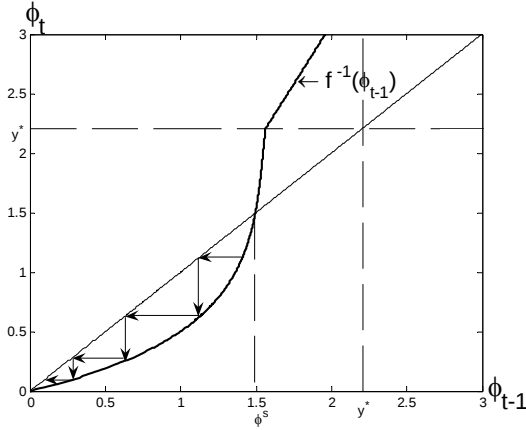
Figure 4-1: Nonstationary equilibria
