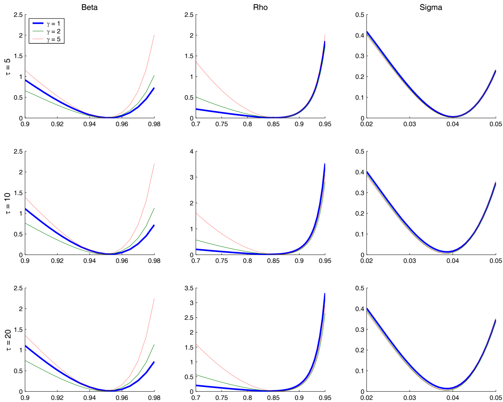
Figure 5: Objective Functions
