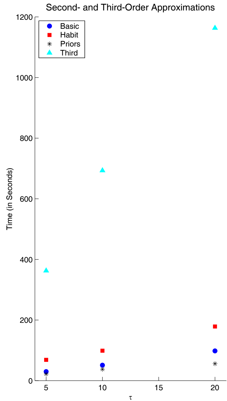
Figure 10: Computing Time
