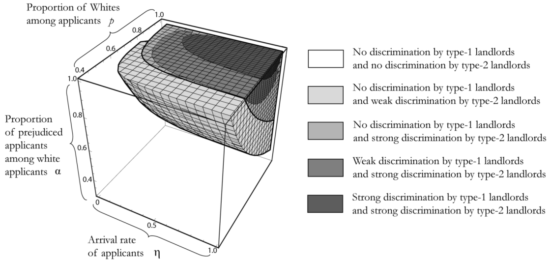
Figure 1: Triplets \{p, \alpha, \eta\} for which discrimination is a dominant strategy
