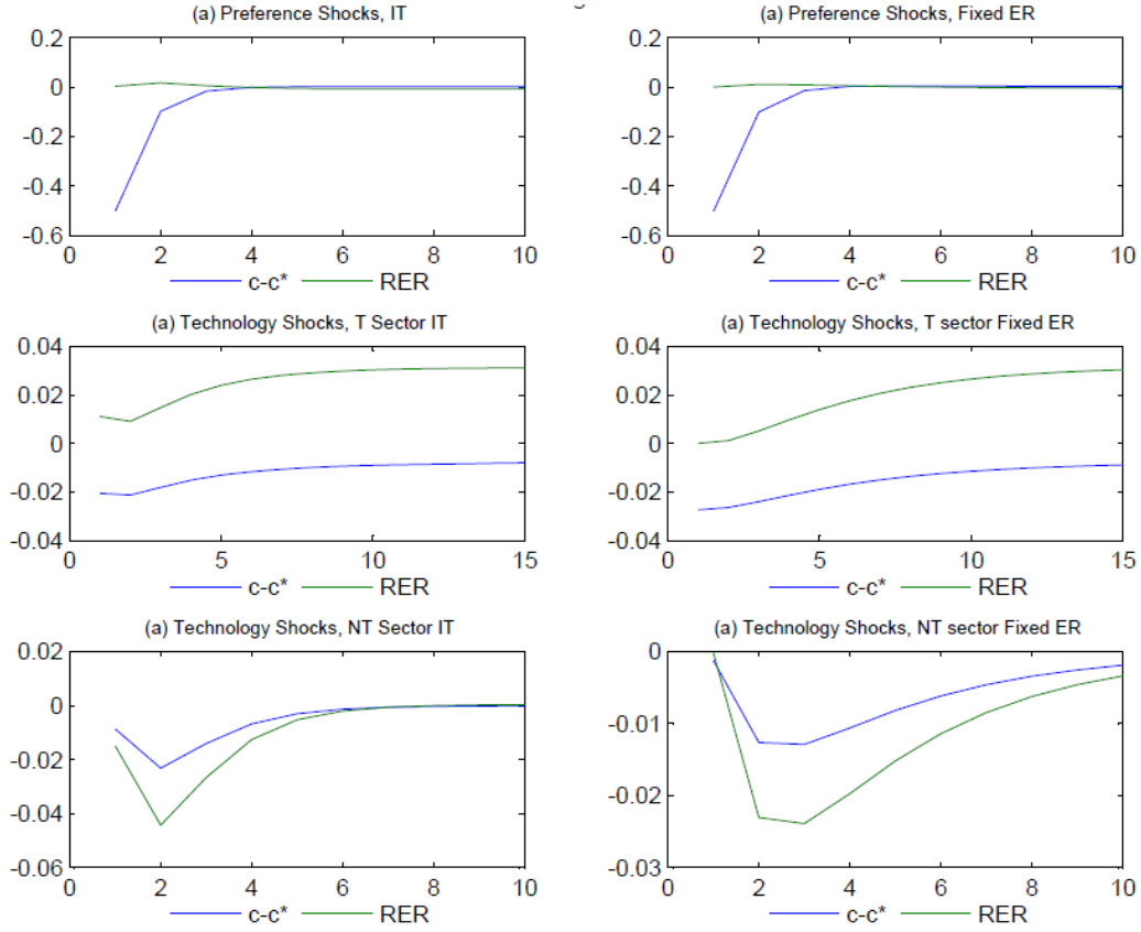
Figure 3: Impulse responses in the extended model
