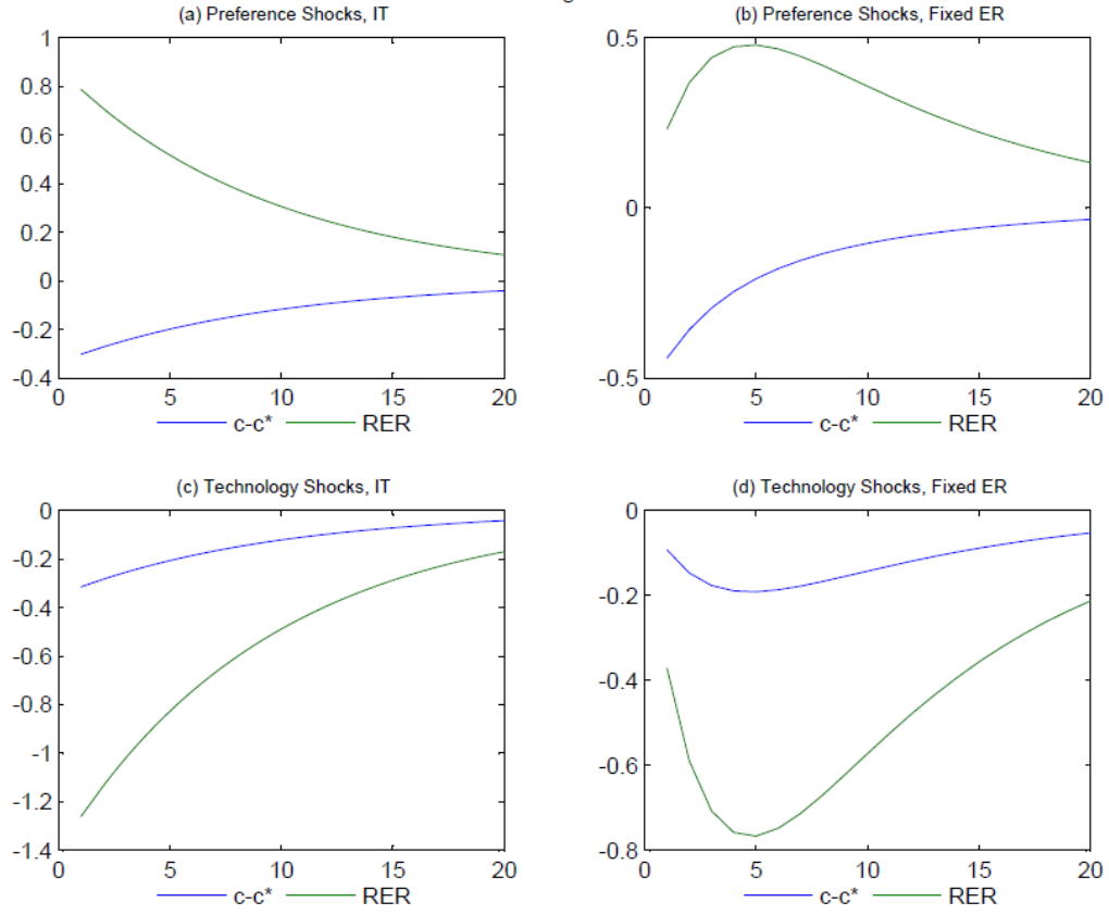
Figure 1: Impulse responses in the bare-bones model
