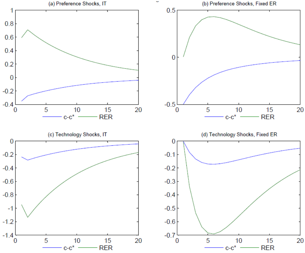
Figure 2: Impulse responses in the bare-bones model with ex-ante pricing
