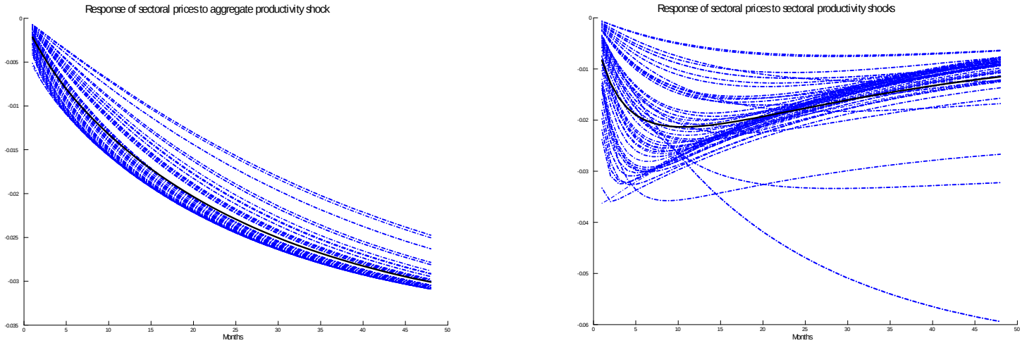
Figures 13-14: Theoretical IRFs
