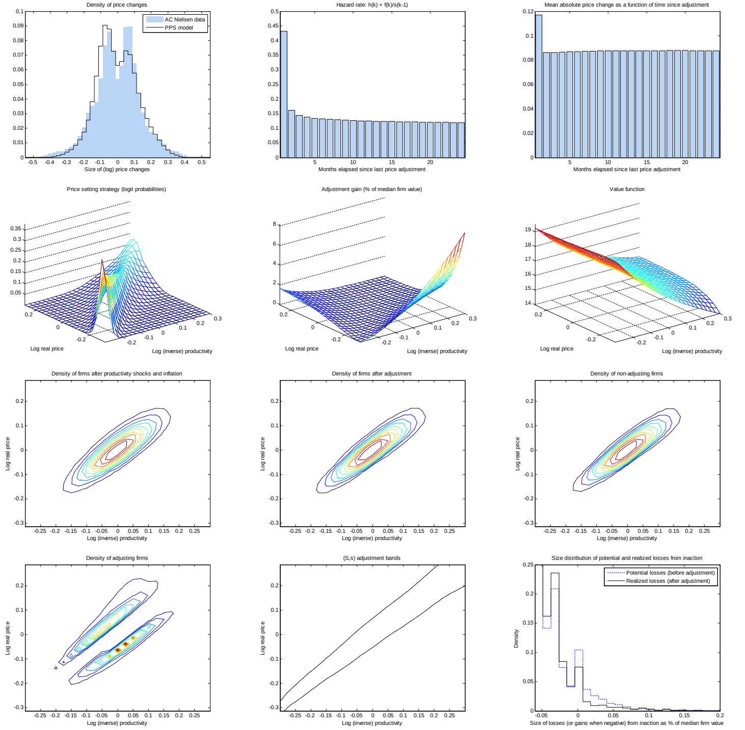
Figure 1. Steady-state value function, distributions, and related objects
