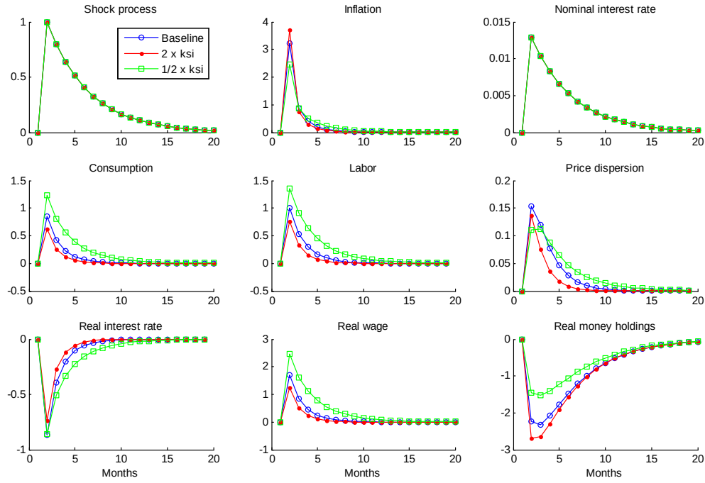
Figure 2. Impulse-response functions: correlated money growth shock
