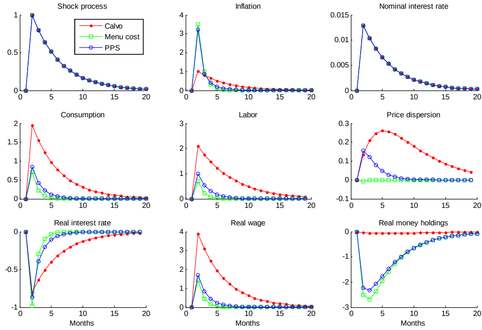
Figure 3. Impulse-response functions for alternative models: correlated money growth shock Panels 1-3, 7: percentage points difference from steady state. Rest of panels: percent deviation from steady state
