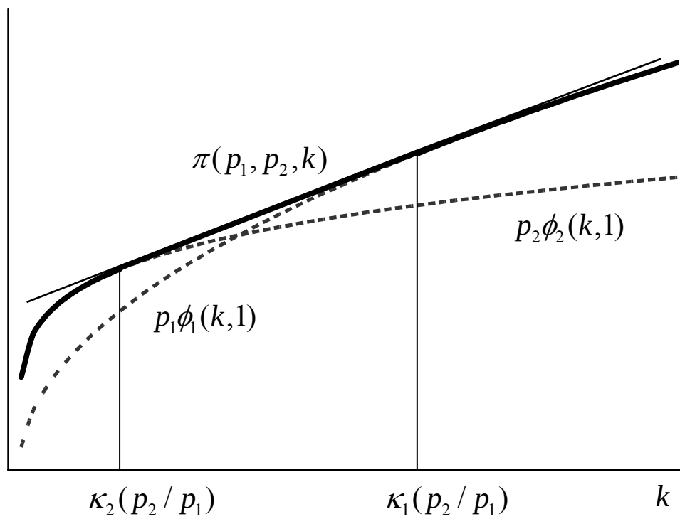
Figure 2. Revenue function
