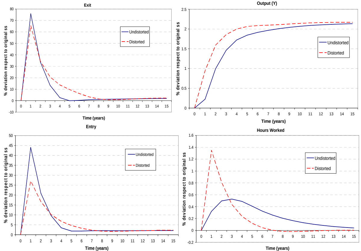
Figure 6. Impulse Responses
