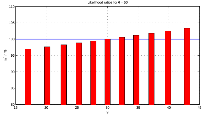
Figure 3: Conditional likelihood ratios m^* for \theta = 50 ( \sigma = -0.02 ).
